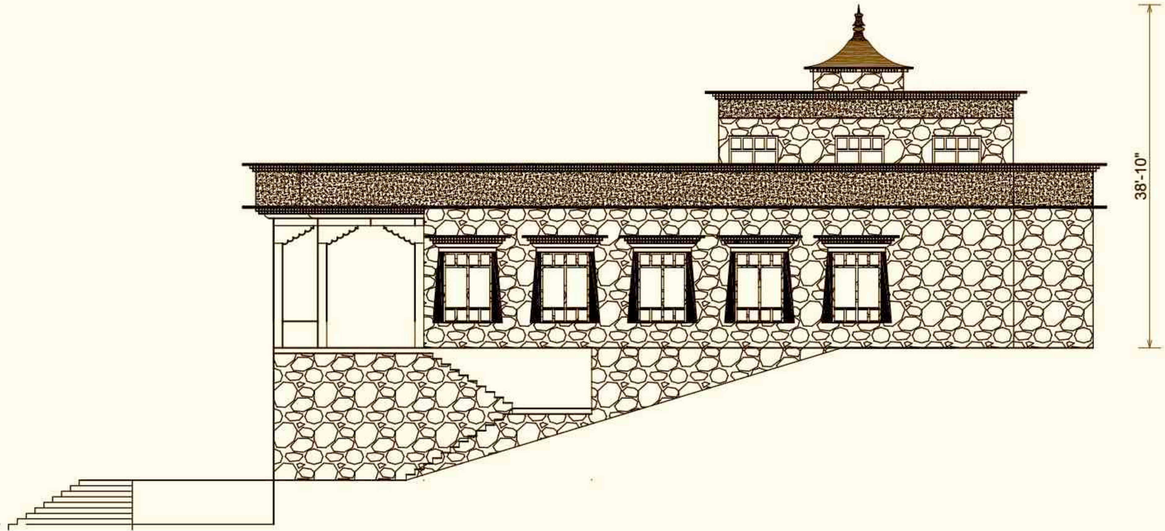
SIDE ELEVATION
