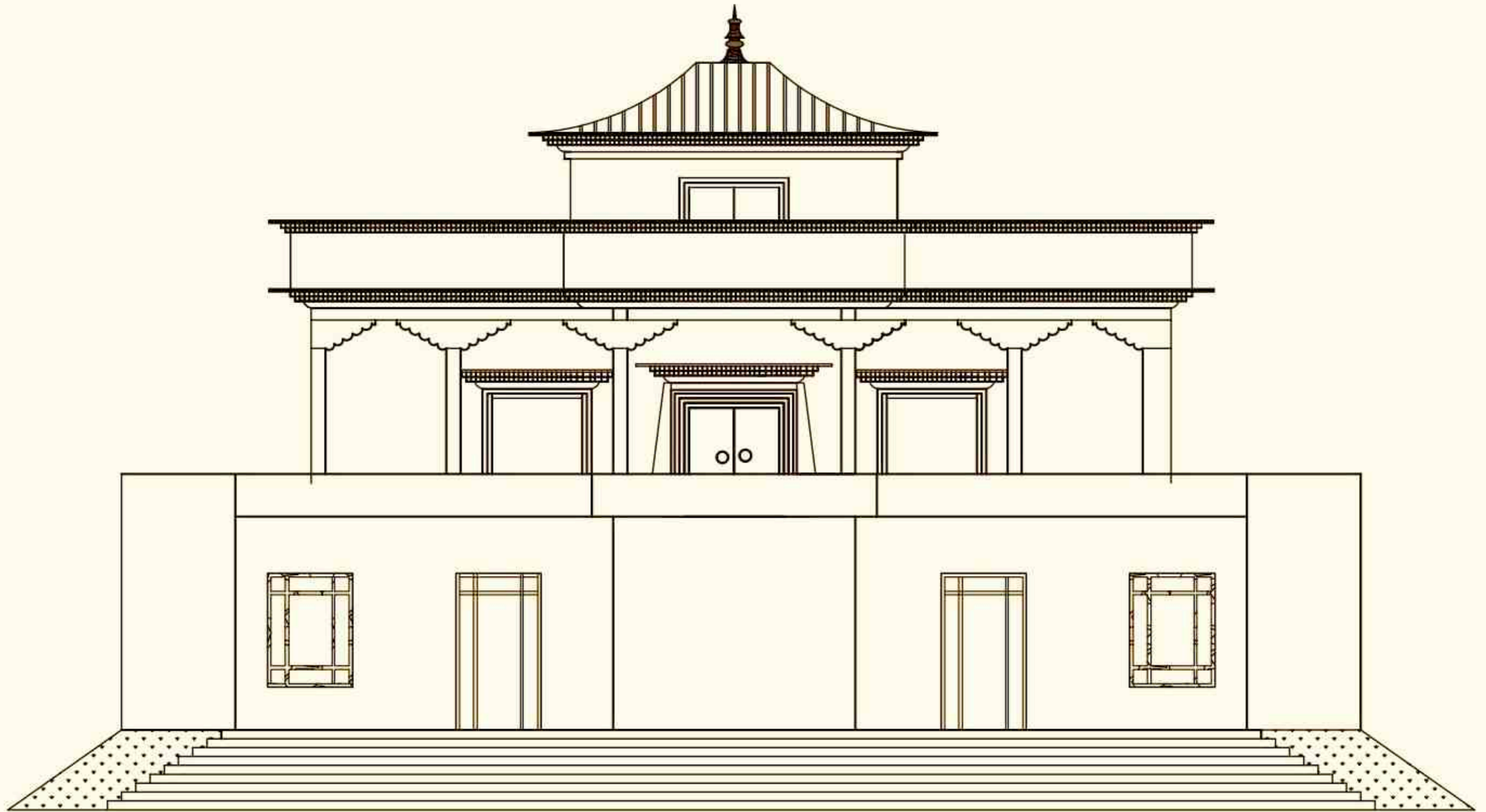
FRONT ELEVATION
